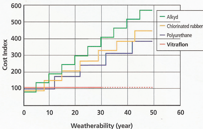
Life Cycle Costs of Vitraflon & Other Coatings
