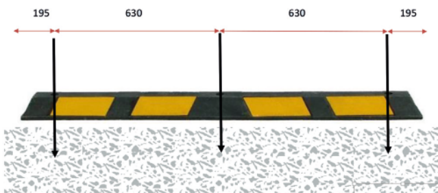
CONCRETE FIXING (removable)
