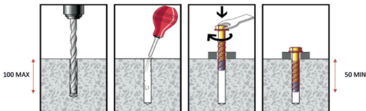
ASPHALT FIXING Method 1
