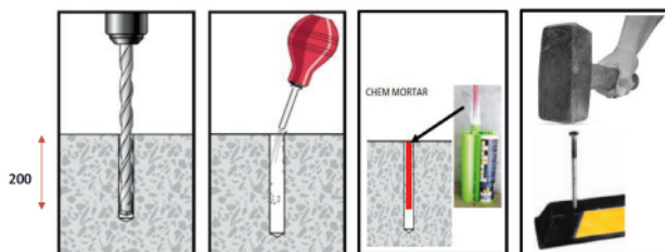
ASPHALT FIXING Method 2
